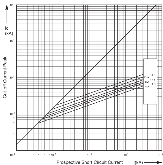
Cut-Off Characteristics
