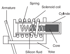
Fig. 2 Overcurrent
