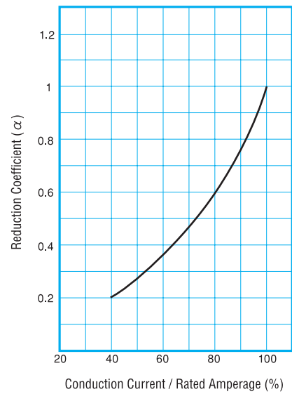
Application to Direct-Current Circuit
